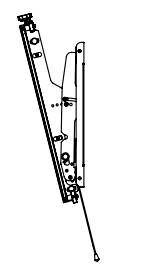
SIDE VIEW 15° Tilt (MAX)
