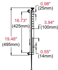
ADAPTOR BRACKET DETAIL
